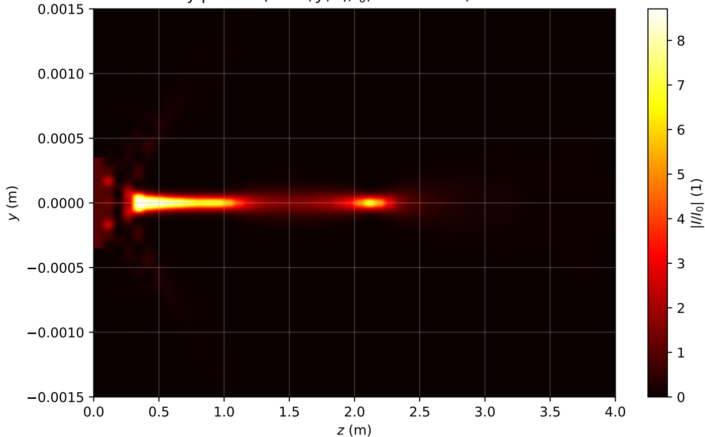
Intensity profile I(x=0, y, z)/I_0 , P_{in}=8.0P_{cr} , artificial time
